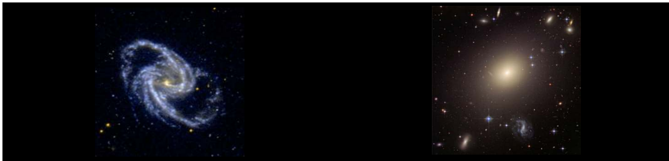
6.18 - A Spiral galaxy
